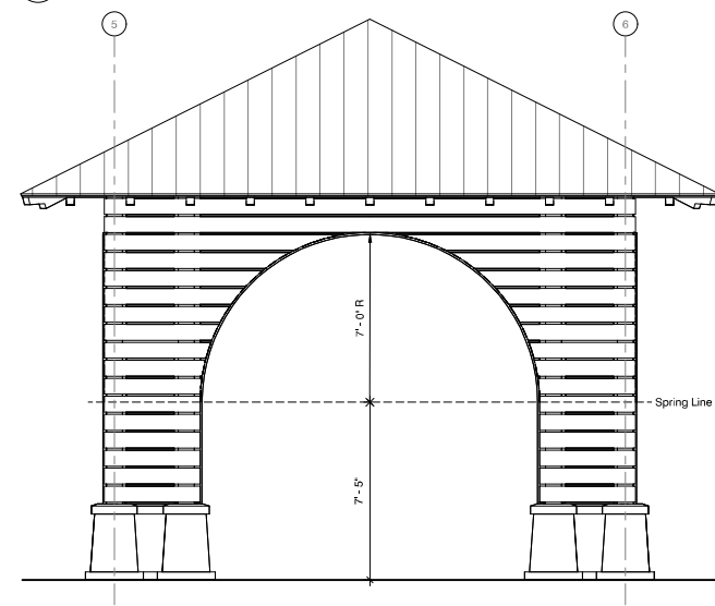
3 Pavilion 2 Elevation 3/8" = 1'-0"
