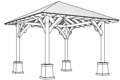
5 Pavilion 1 3D
