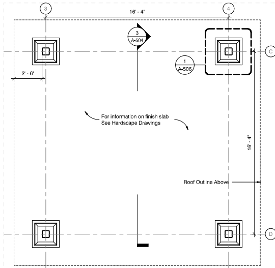
1 Pavilion 1 Plan 3/8" = 1'-0"
