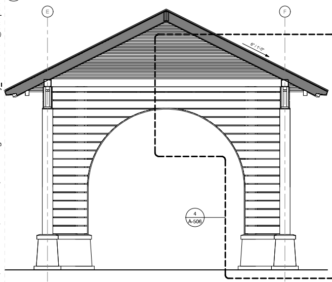
4 Pavilion 2 Section 3/8" = 1'-0"
