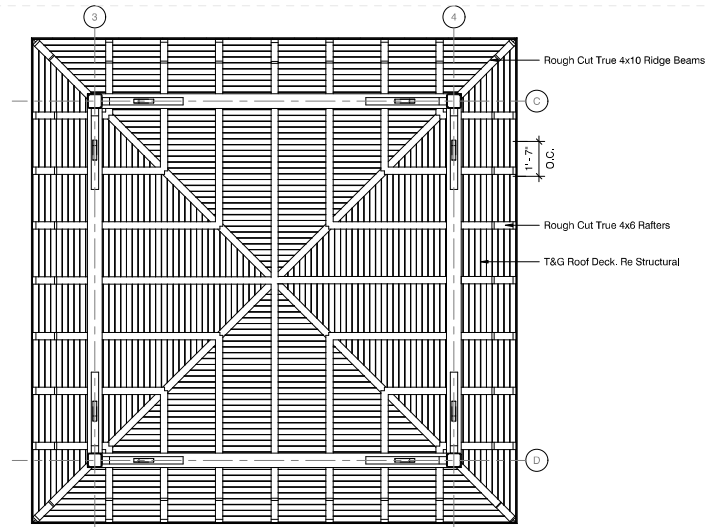
2 Pavilion 1 RCP 3/8" = 1'-0"
