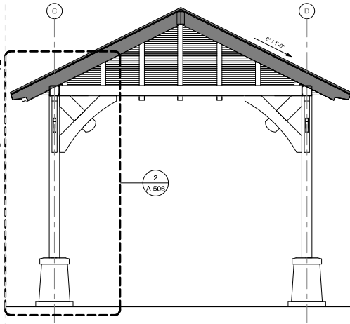
3 Pavilion 1 Section 3/8" = 1'-0"
