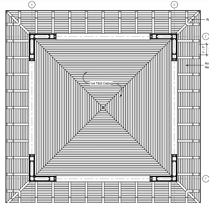
2 Pavilion 2 RCP 3/8" = 1'-0"
