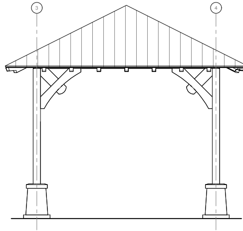
4 Pavilion 1 Elevation 3/8" = 1'-0"
