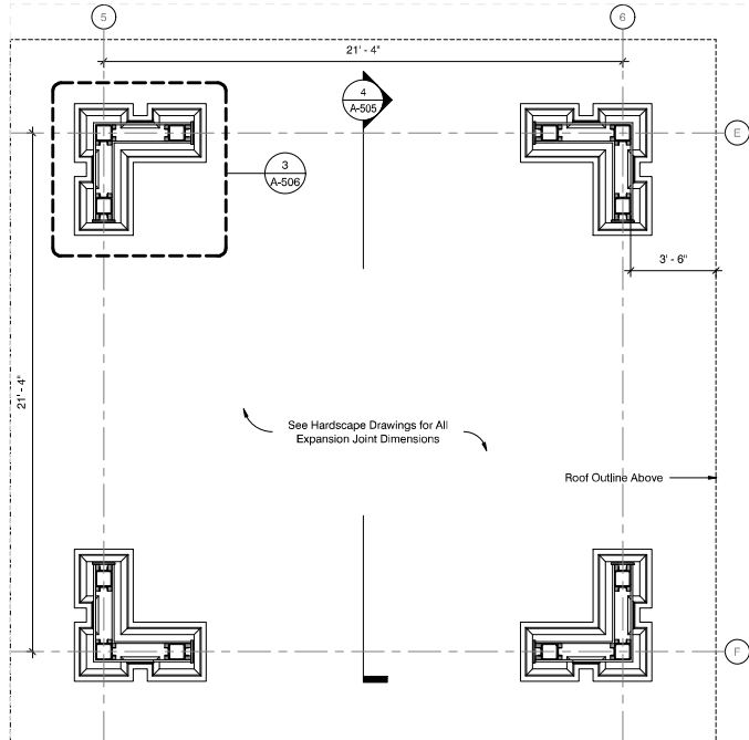
1 Pavilion 2 Plan 3/8" = 1'-0"
